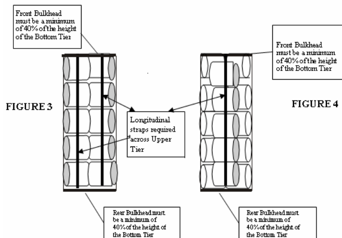
Figure 3 &amp; 4 - Load on Farm Wagons
