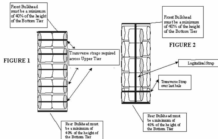
Figure 1 &amp; 2 - Loads on Commercial Vehicles other than Farm Wagons
